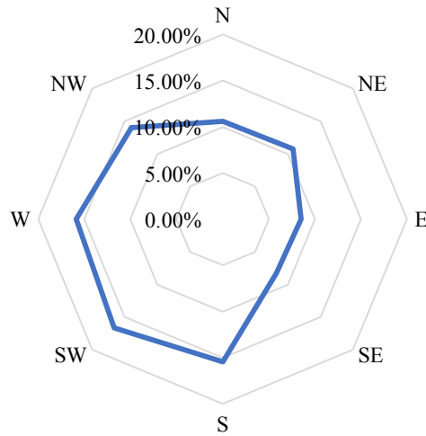
Figure C.22: Wind rose for the 6X6 square wind farm, 8D spacing, with a 9° orientation.
