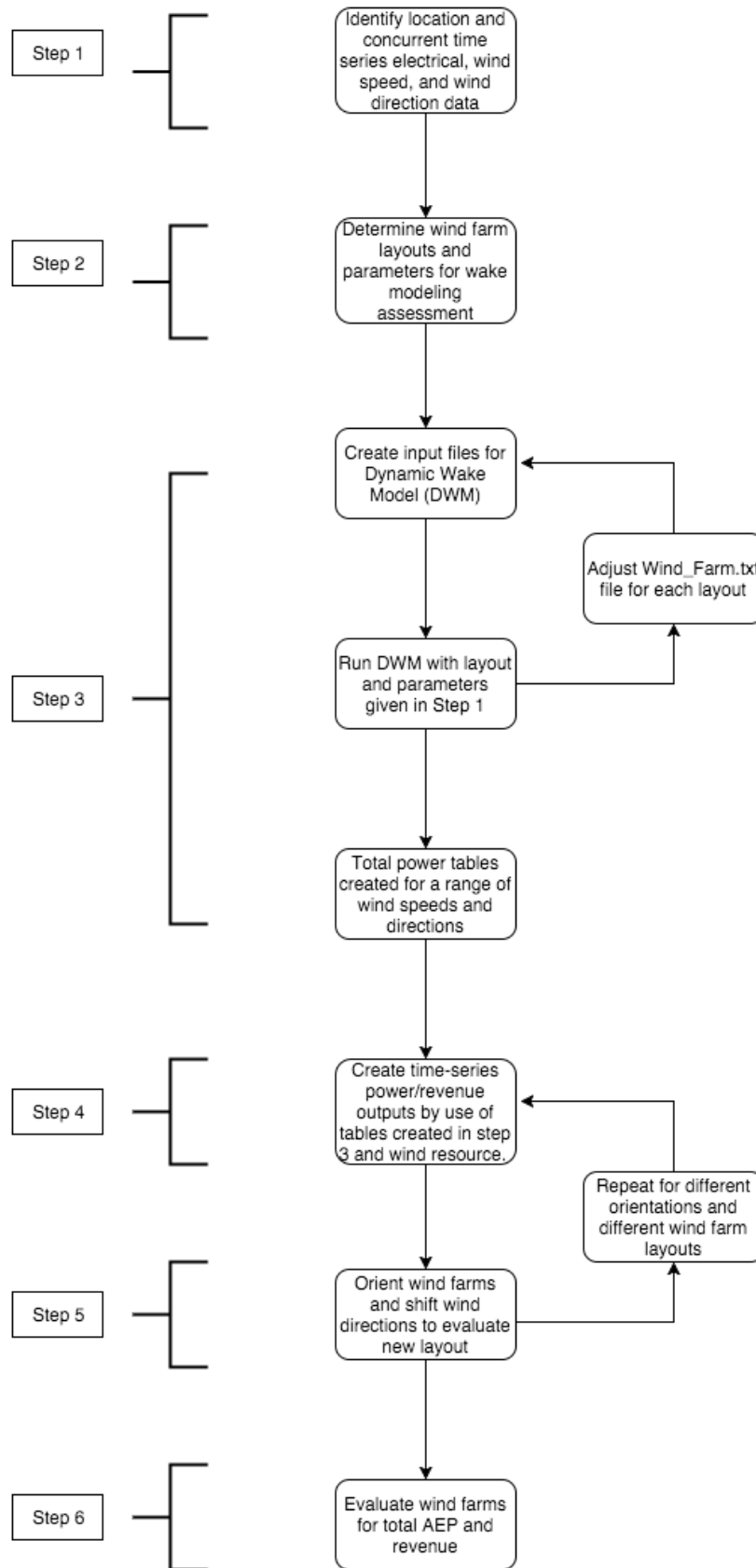
Figure 3.1: Flow chart of the micrositing process.
