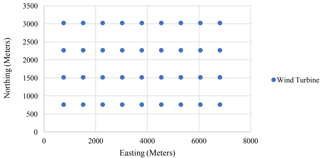
9X4 Rectangle Wind Farm with 6D Spacing
