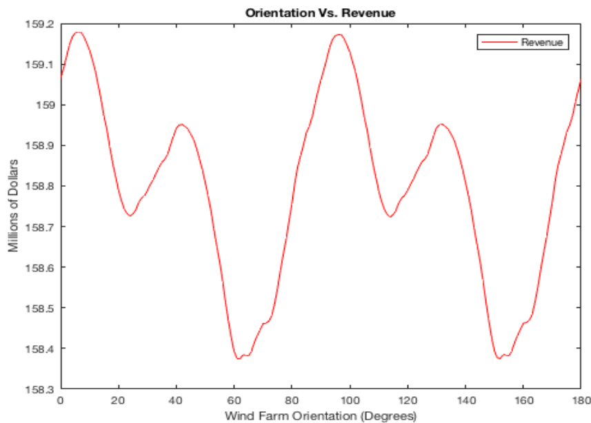
Figure 4.20: Revenue for the 6X6 square wind farm with 6D spacing.
