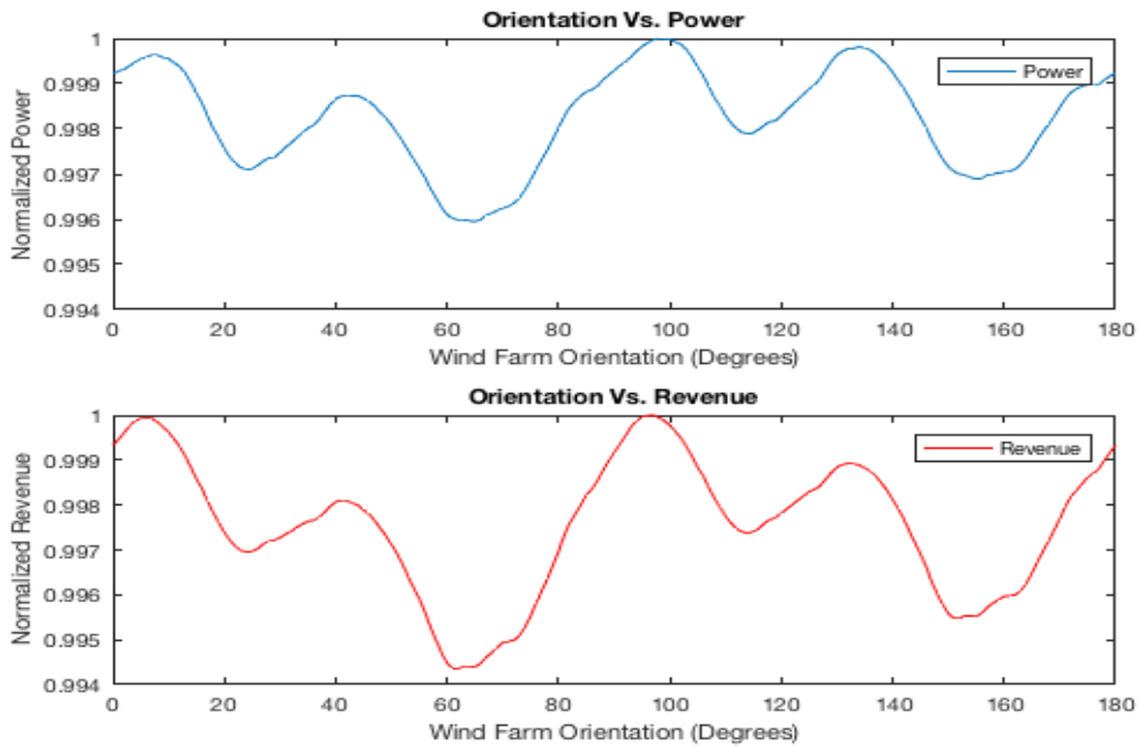
Figure C.4: Relationship between the total revenues and total powers for the 9X4 rectangular wind farm with 6D spacing.
