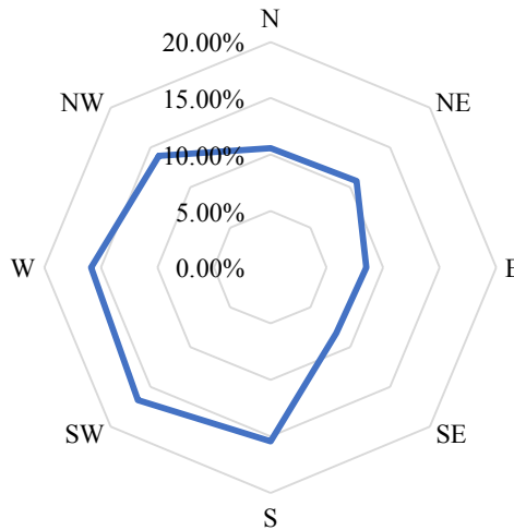
Figure C.6: Wind rose for the 9X4 rectangular wind farm when the orientation is 95°.
