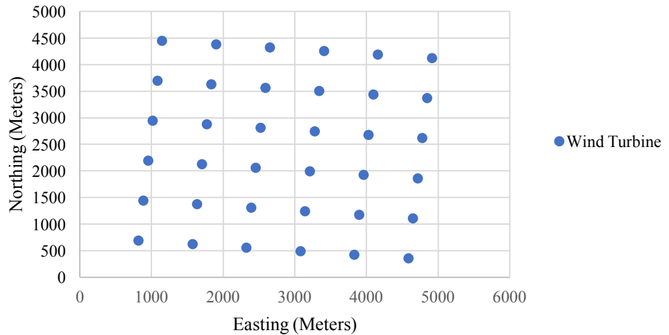
Figure 4.23: 6X6 square wind farm with a 5^\circ orientation.
