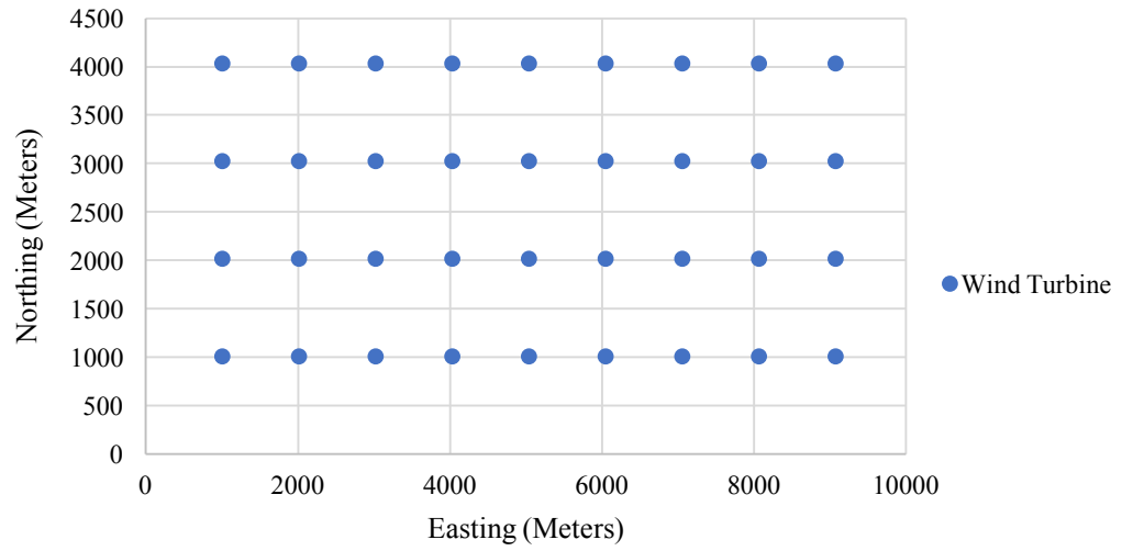
Figure 3.6: 9X4 rectangular wind farm with 8D spacing.
