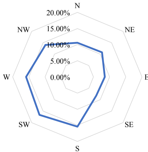
Figure C.8: Wind rose for the 9X4 rectangular wind farm when the orientation is 61°.
