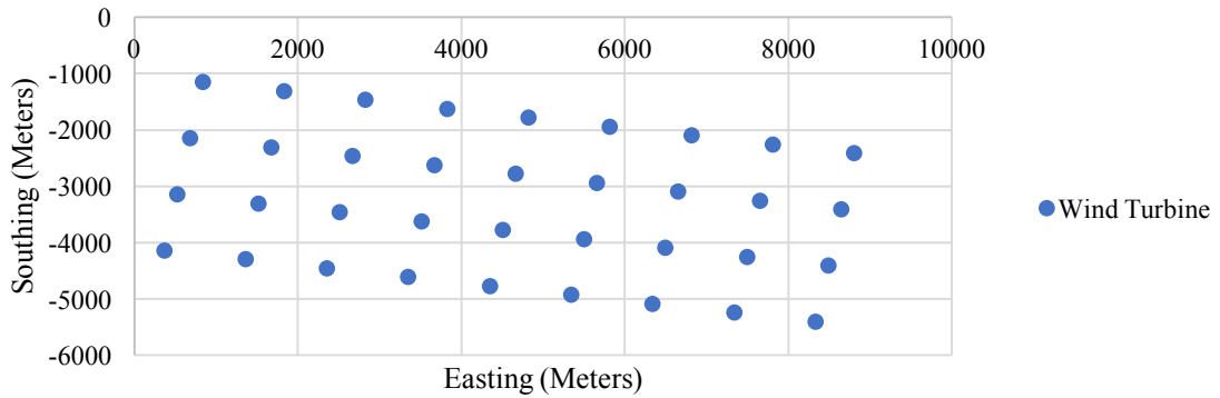
Figure C.29: 99° orientation that maximizes power and revenue for the candidate wind farm.
