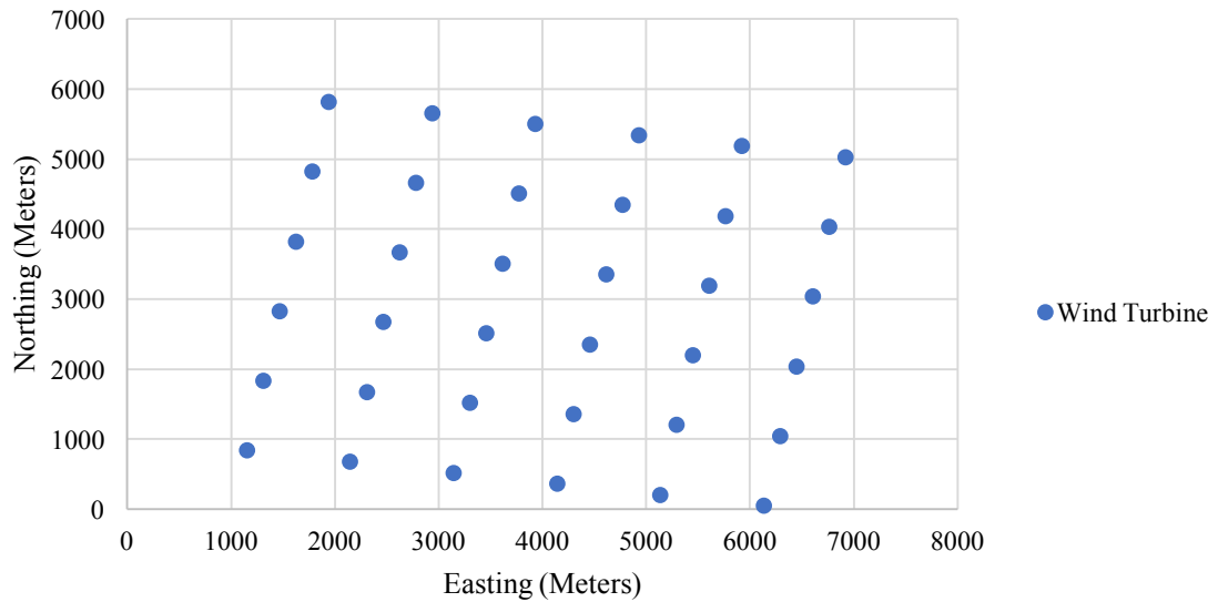
Figure C.21: 6X6 square wind farm, 8D spacing, with a 9° orientation to maximize power and revenue.
