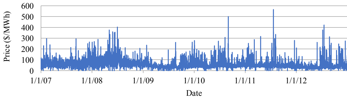
Figure 3.17: 5-year time-series price and power data from Southeastern Massachusetts, including Nantucket.
