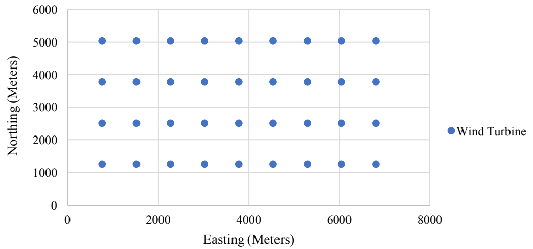
Figure 3.7: 9X4 rectangular wind farm with 6D and 10D spacing.
